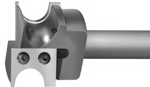
Multiprofile Bull Nose Insert Body
